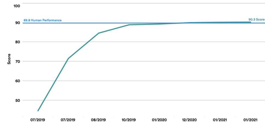
SUPERGLUE BENCHMARK Source: SuperGLUE Leaderboard, 2020 | Chart: 2021 AI Index Report
