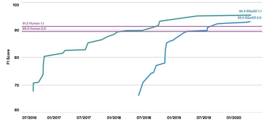
SQUAD 1.1 and SQUAD 2.0: F1 SCORE Source: CodaLab Worksheets, 2020 | Chart: 2021 AI Index Report
